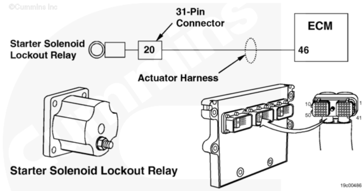
Starter Solenoid Lockout Relay Circuit
