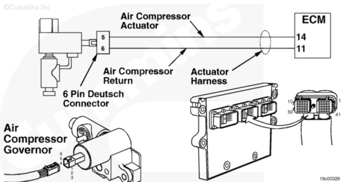
Electronic Air Compressor Governor Circuit
