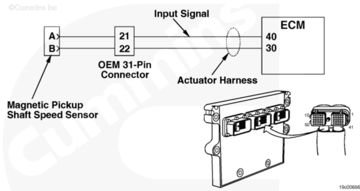
Auxiliary Speed Input Circuit
