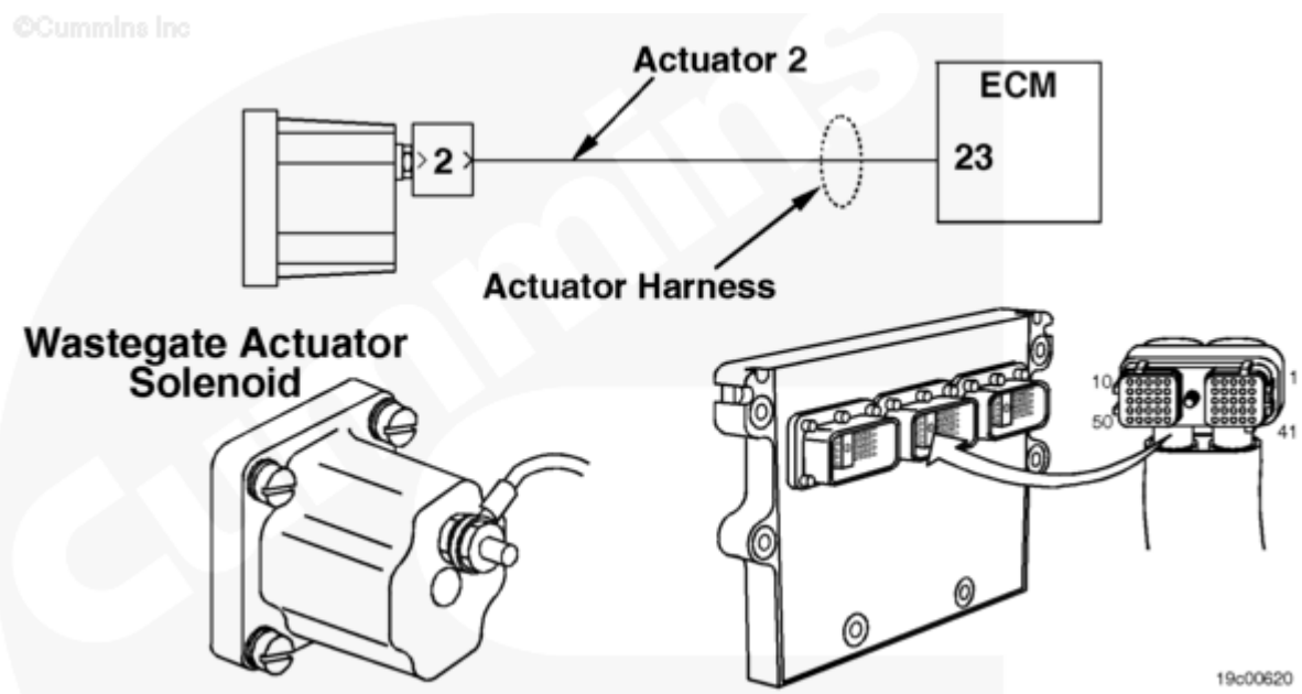
Wastegate Actuator Number 2 Circuit
