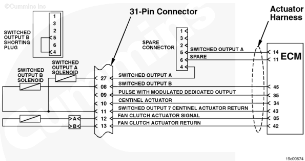
Switched Output A Circuit
