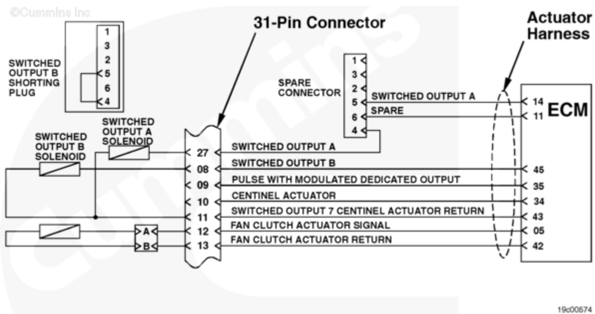
Switched Output B Circuit
