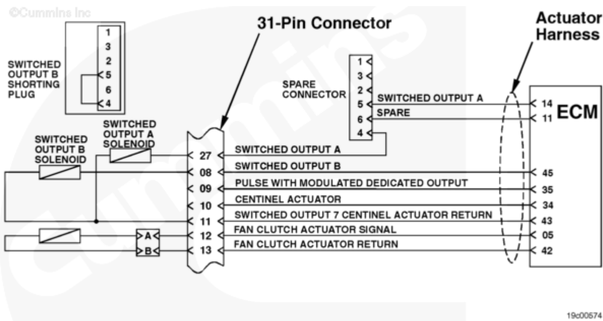
Switched Output B Circuit
