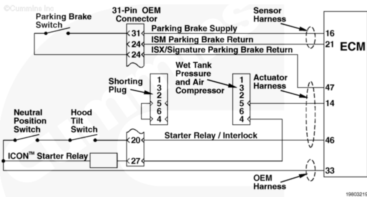
ICON™ Starter Relay/Interlock Circuit
