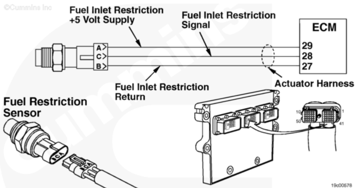
Fuel Inlet Restriction Sensor Circuit
