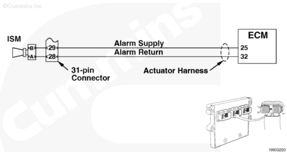
Engine Start Alarm Circuit
