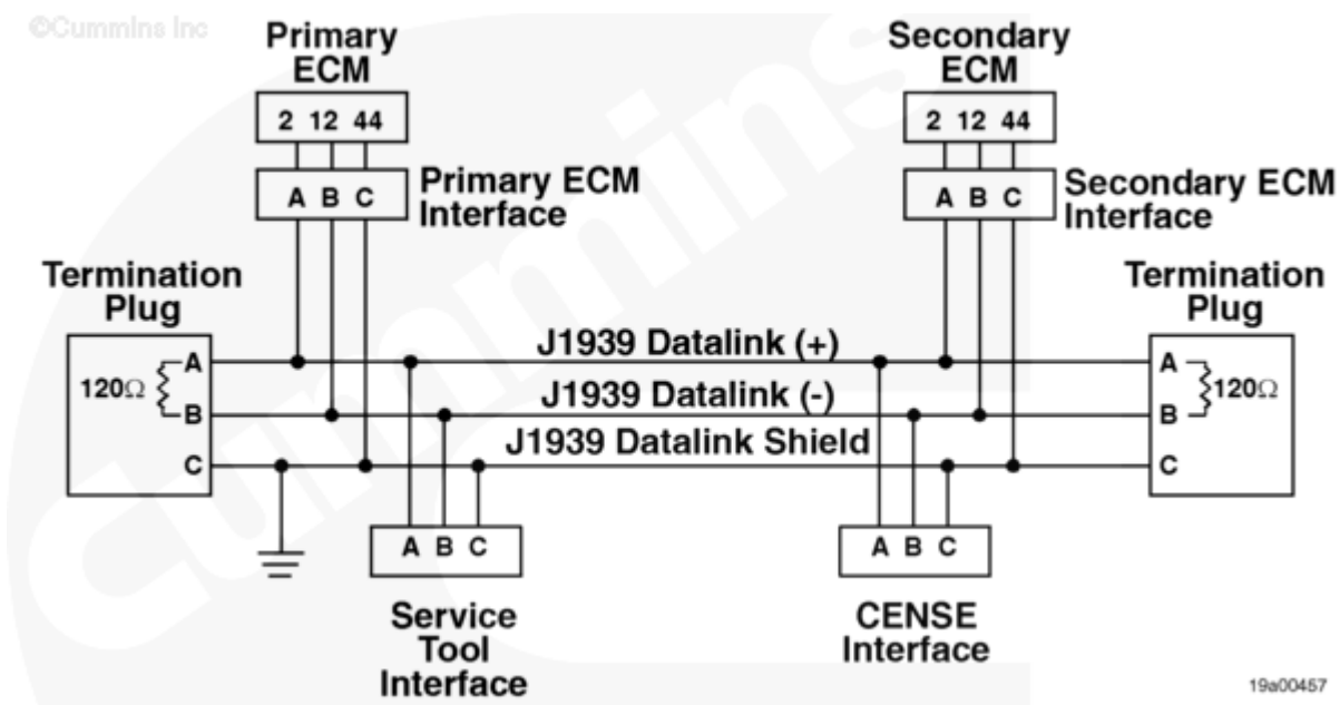
J1939 Backbone Harness Circuit Diagram
