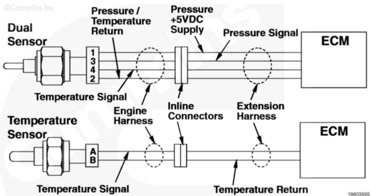
Oil Temperature Sensor Circuit
