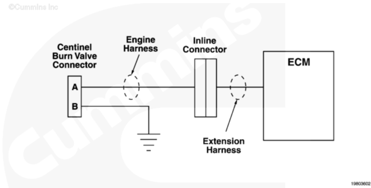
Burn Valve Solenoid Circuit
