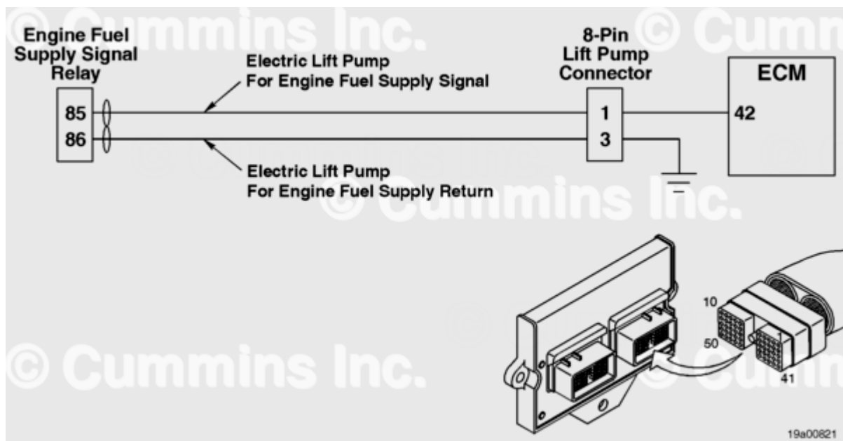
Electric Lift Pump for Engine Fuel Supply Circuit
