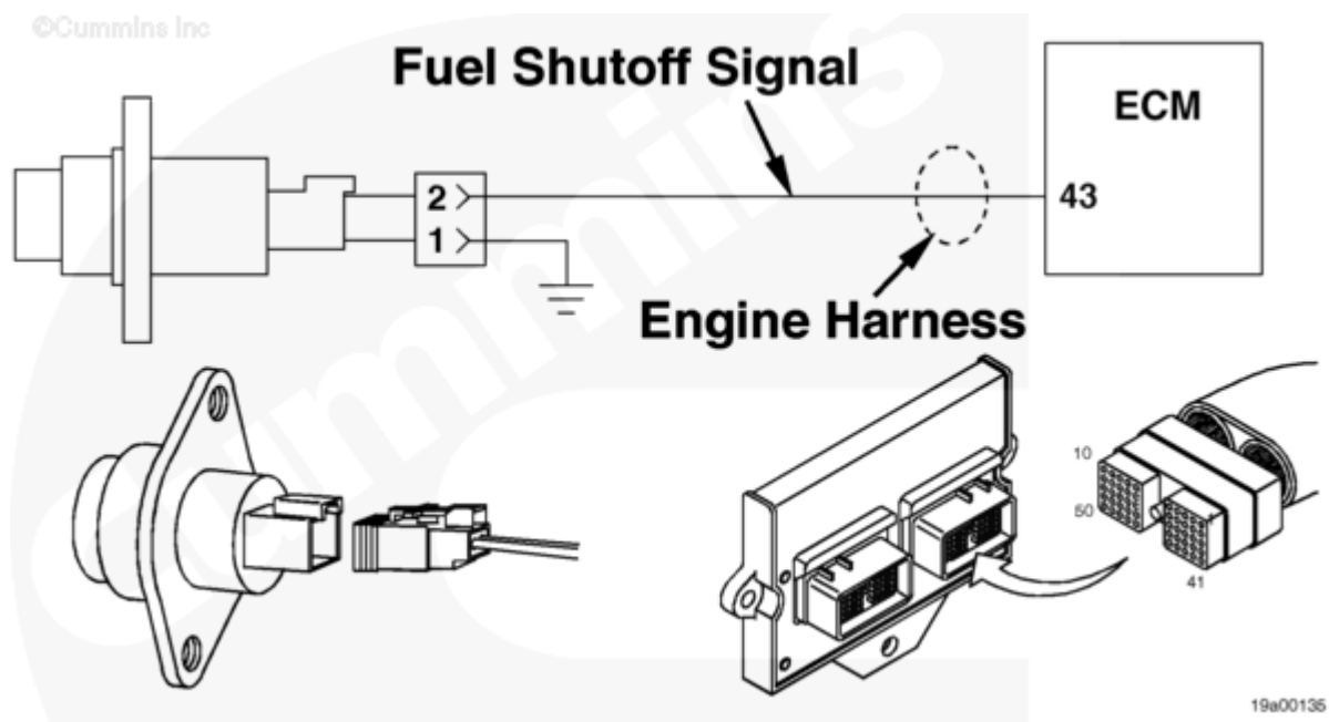
Electrohydraulic Shutoff Device (EHAB) Circuit
