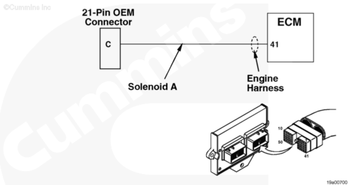
Solenoid A Circuit
