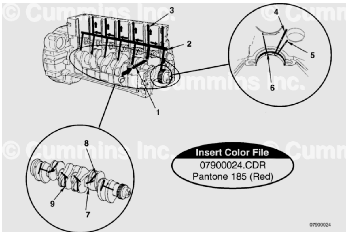
Lubrication for the Power Components
