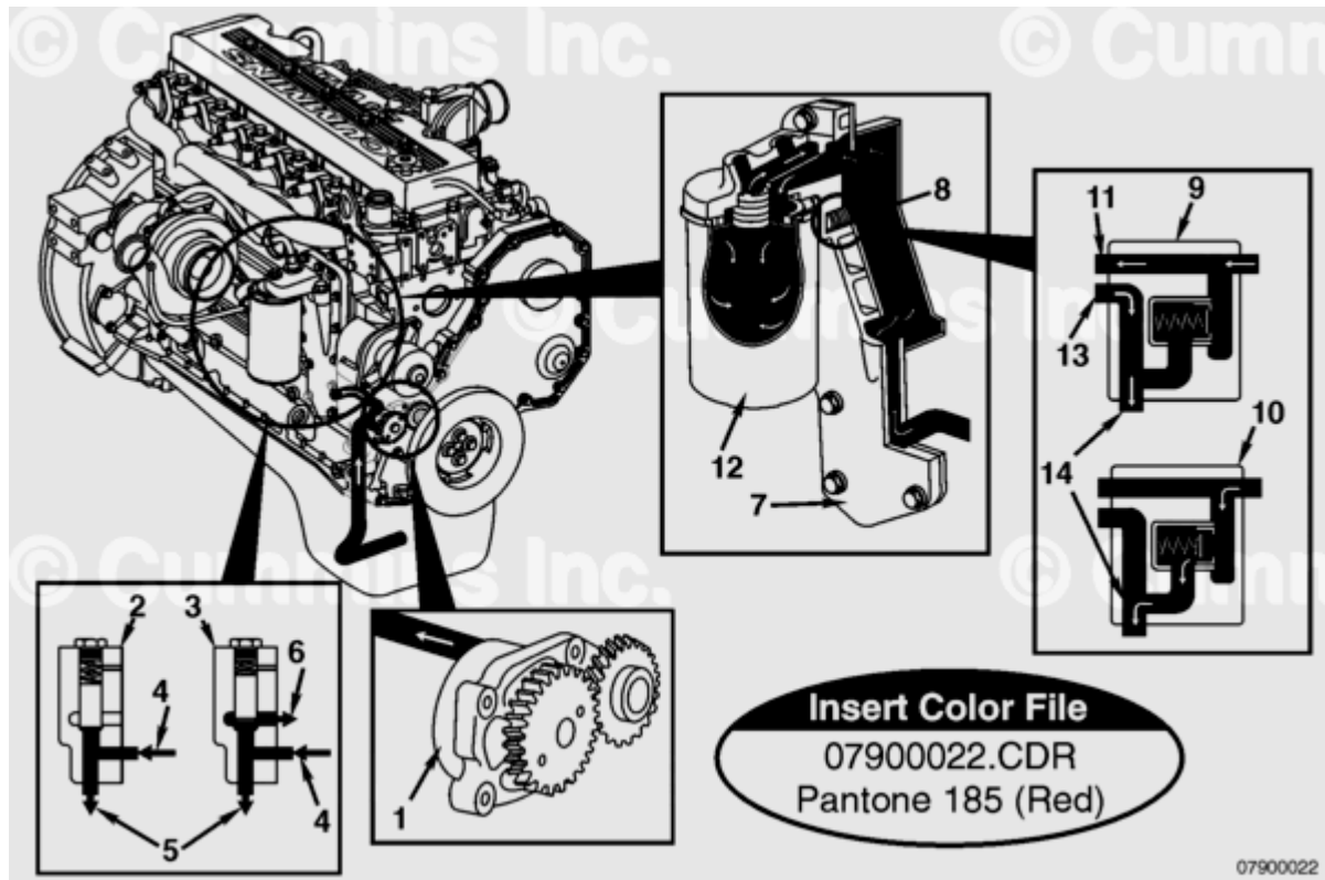
Lubricating Oil Filter and Bypass
