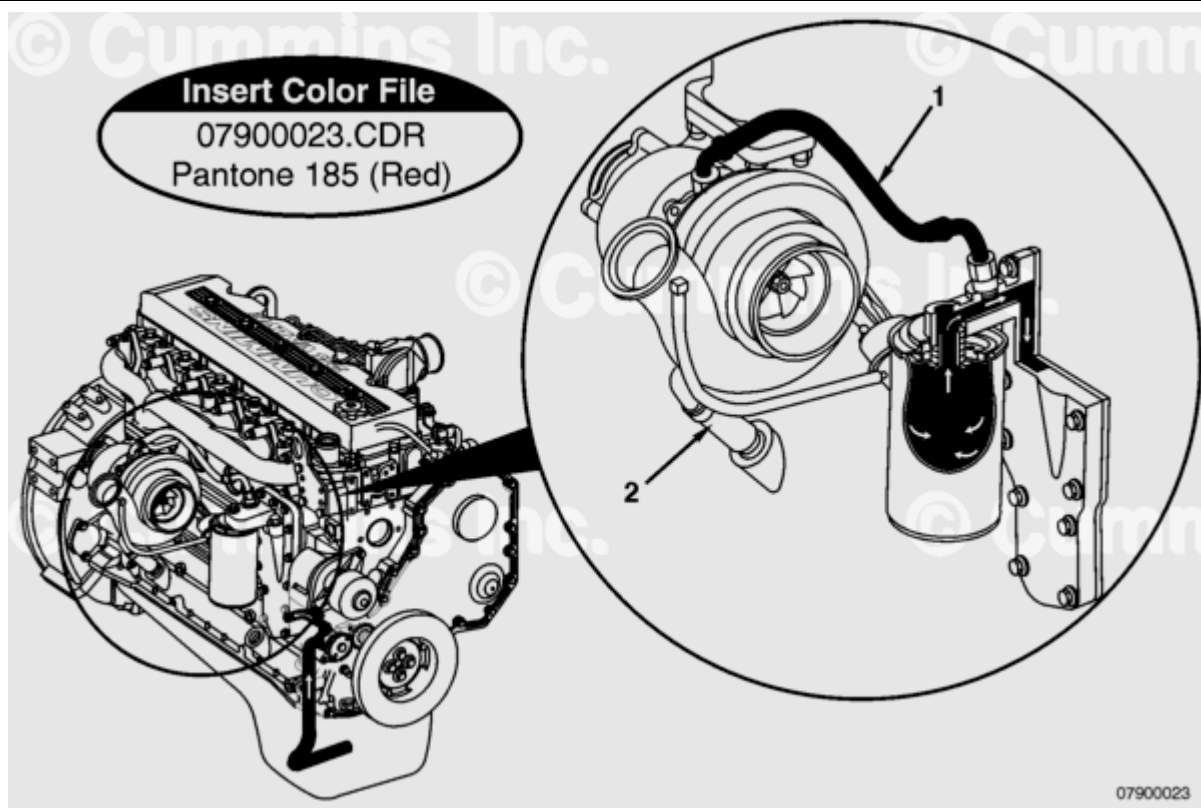
Lubrication for the Oil Turbocharger
