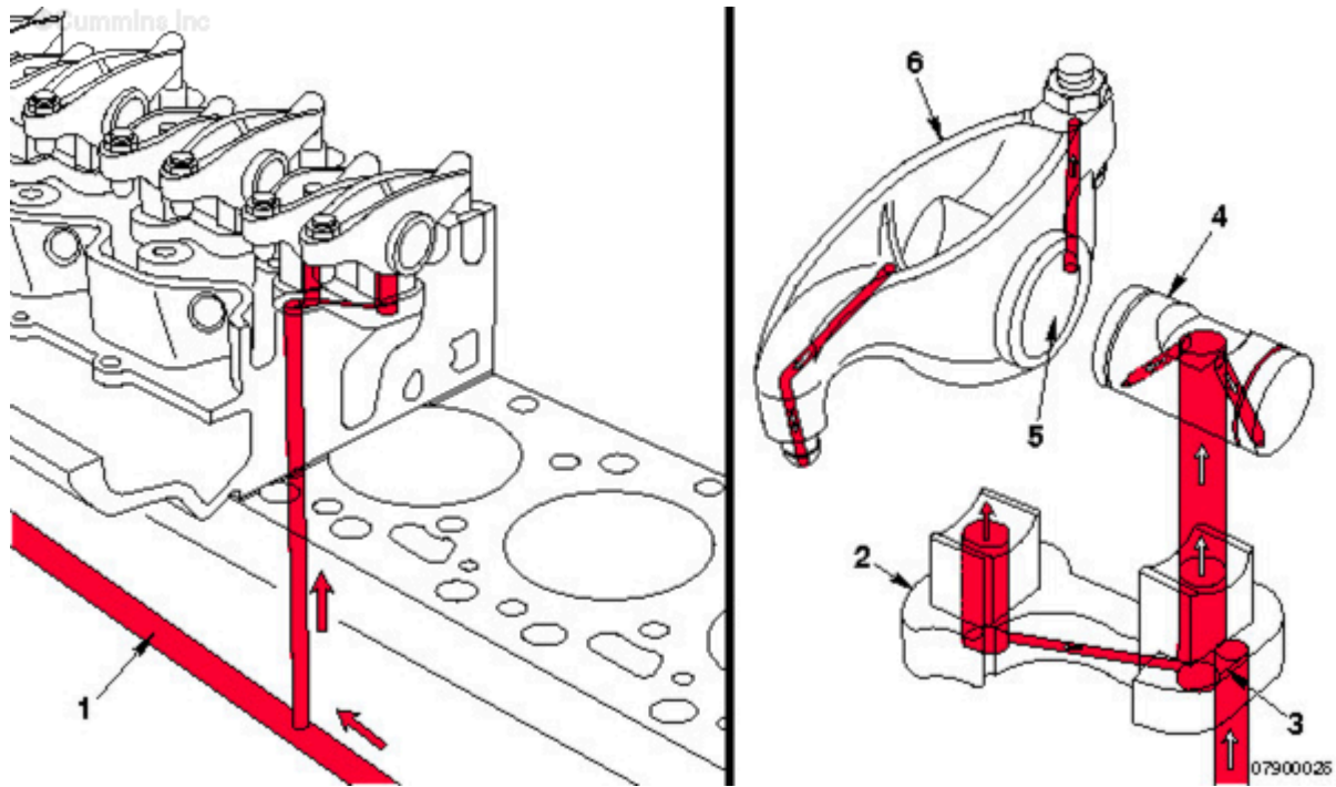
Lubrication for the Overhead
