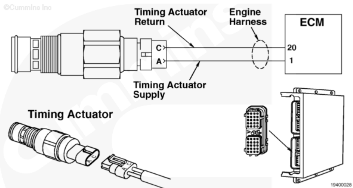
Timing Actuator Circuit
