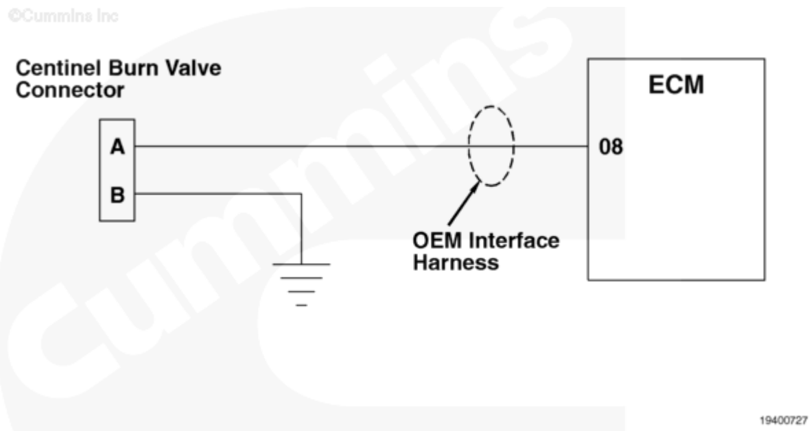
Burn Valve Solenoid Circuit
