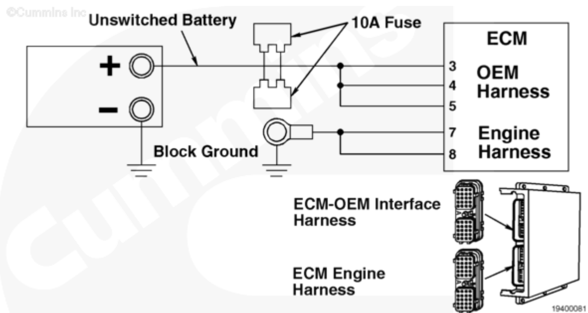
Battery Power and Ground Circuit
