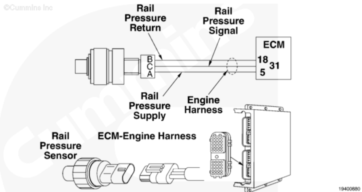
Rail Pressure Sensor Circuit
