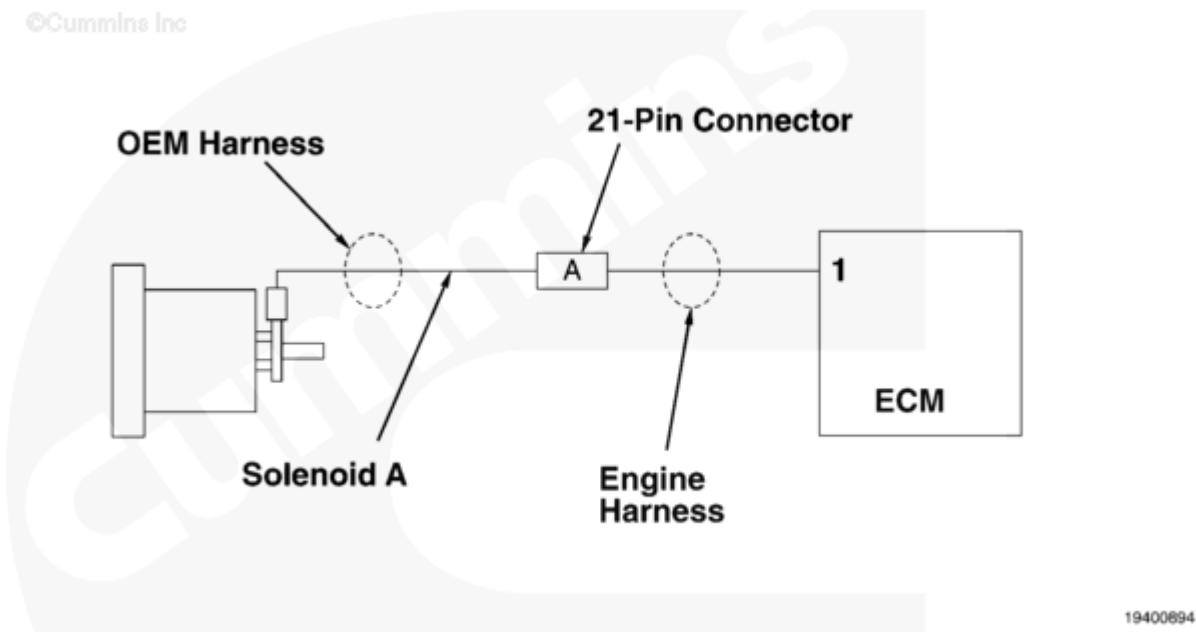
Solenoid A Circuit
