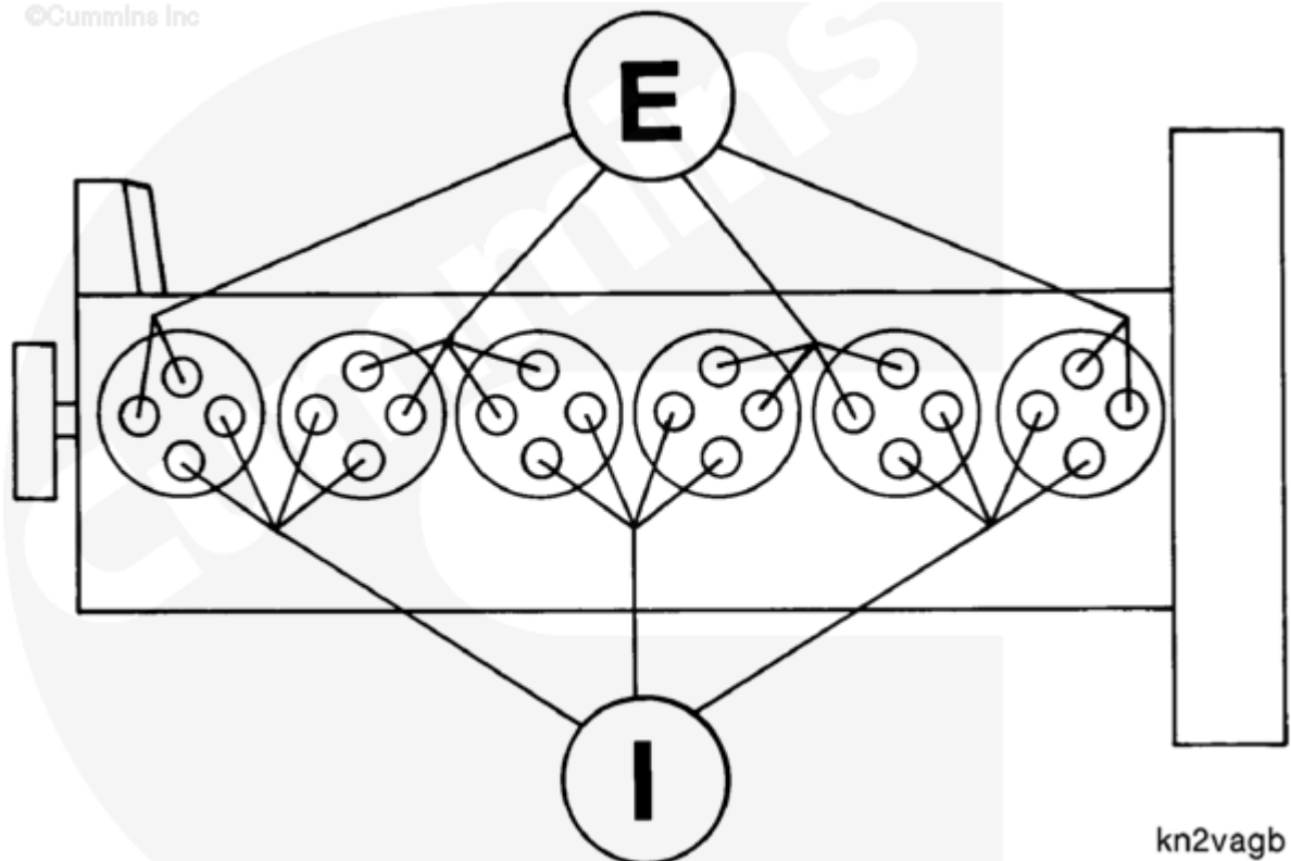
Intake and Exhaust Valve Locations
