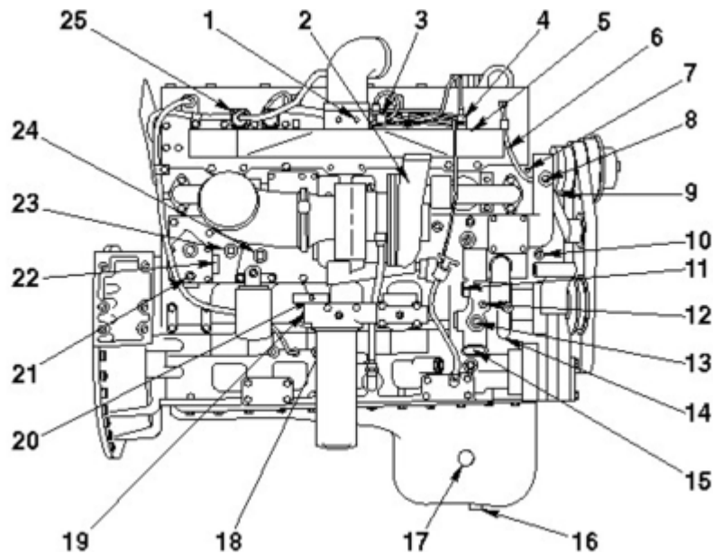
Right View - CM570
