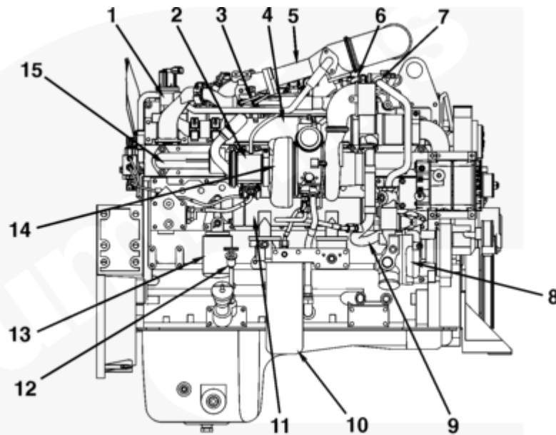
Right - ISM CM876
