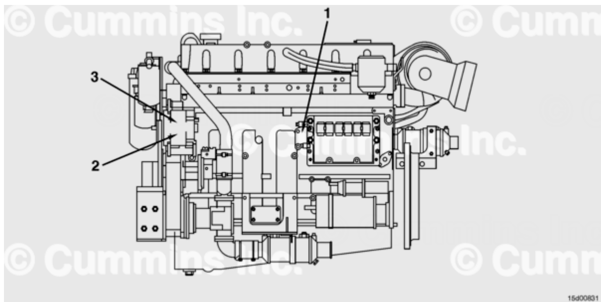
Left (Port) - QSM 11 Marine - Sensors
