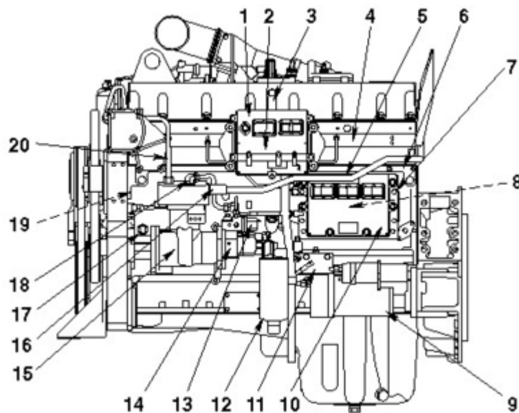
Left View - CM870
