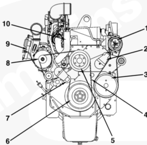
Front - ISM CM876 Automotive
