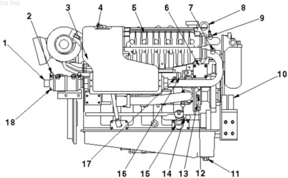
Right (Starboard) - QSM11 Marine - Components
