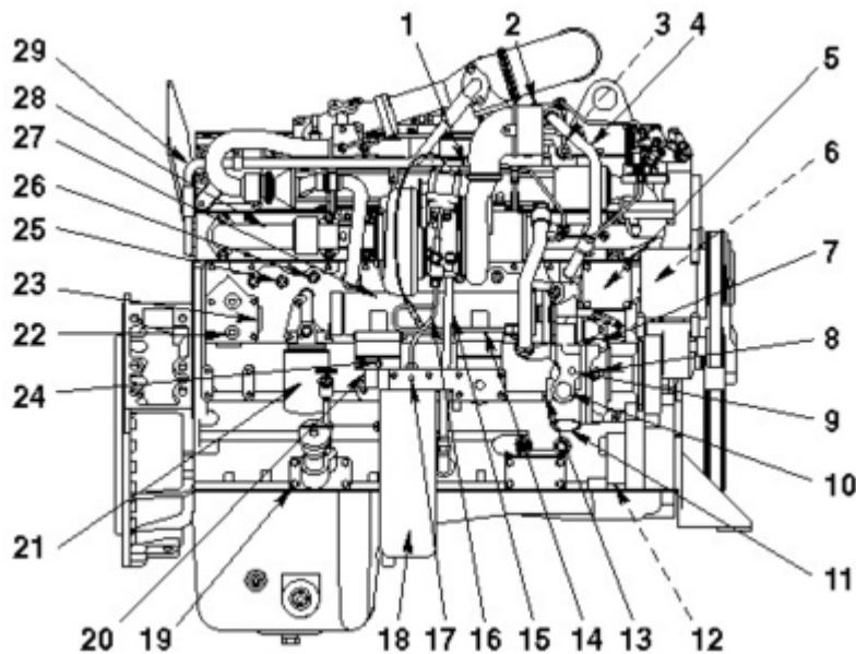
Right - ISM CM870 Automotive
