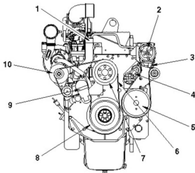
Front View - CM870
