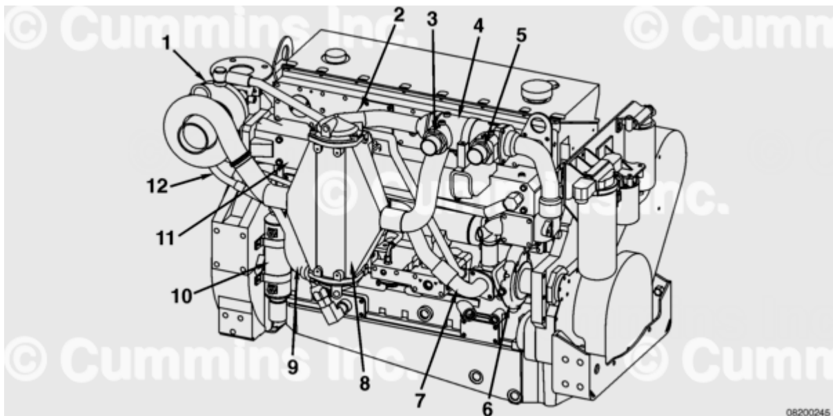
Right (Starboard) - QSM11 Marine - Keel Cooled
