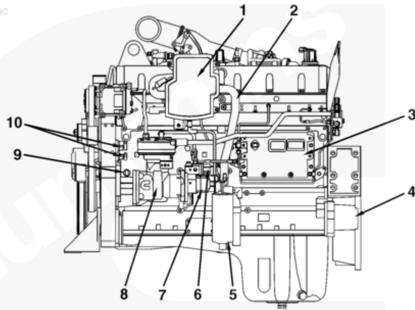
Left - ISM CM876 Automotive
