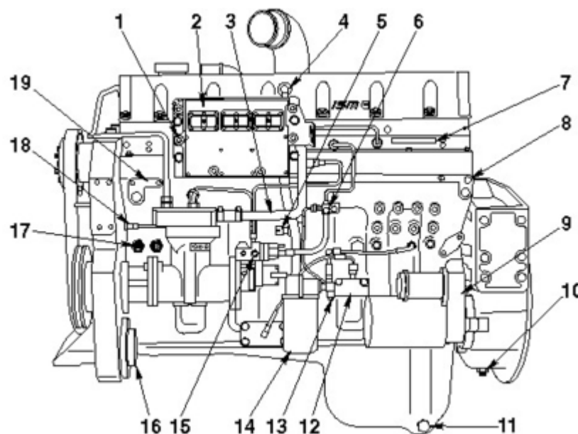
Left View - CM570
