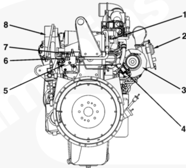
Rear - ISM CM876
