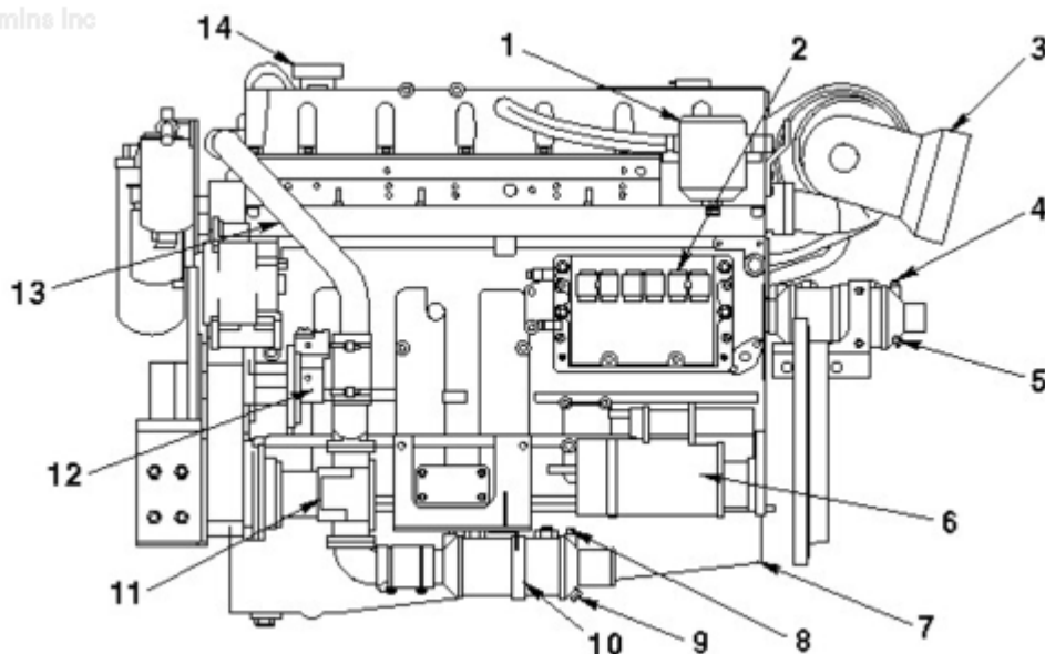
Left (Port) - QSM11 Marine - Components
