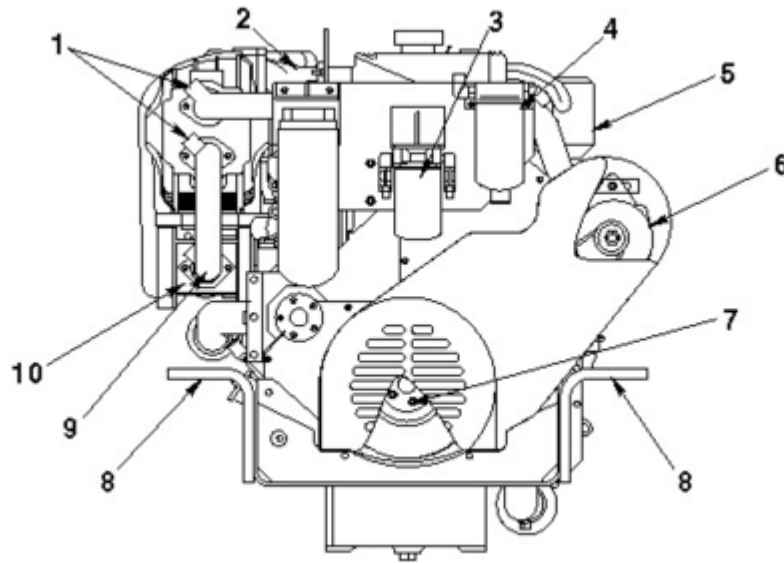
Front - QSM11 Marine
