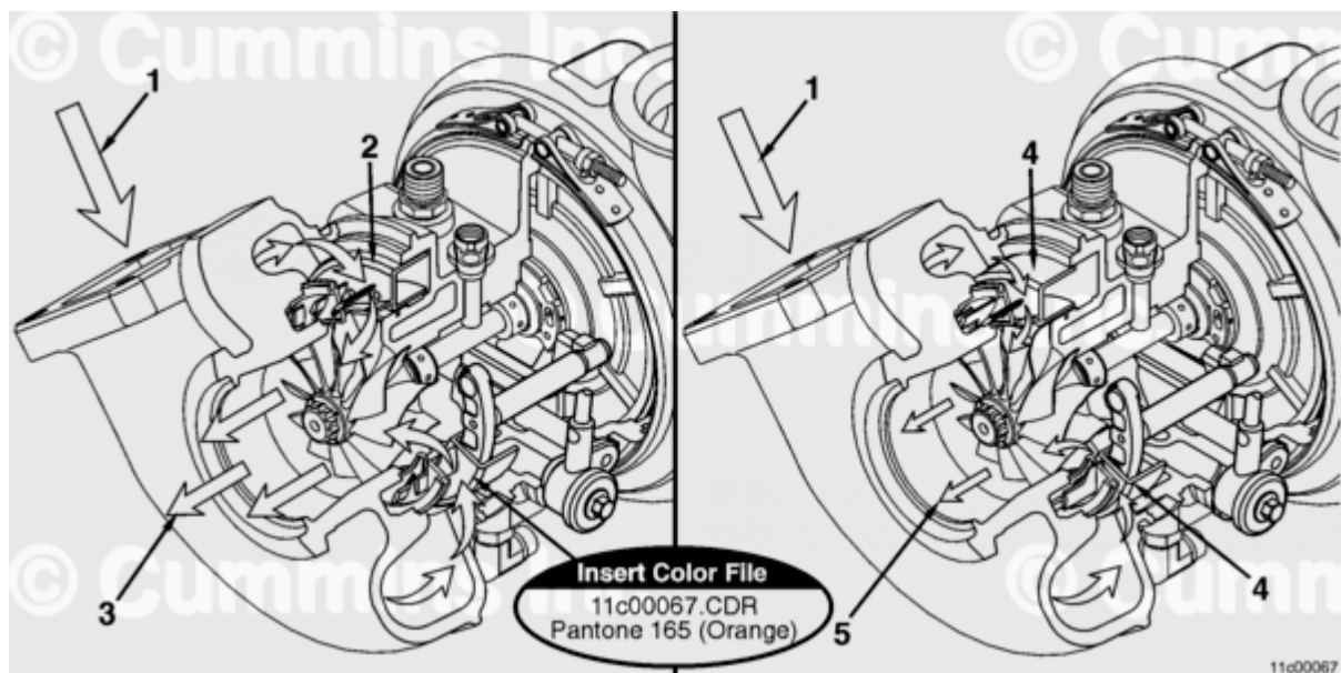
Variable Geometry Turbocharger - Opened and Closed
