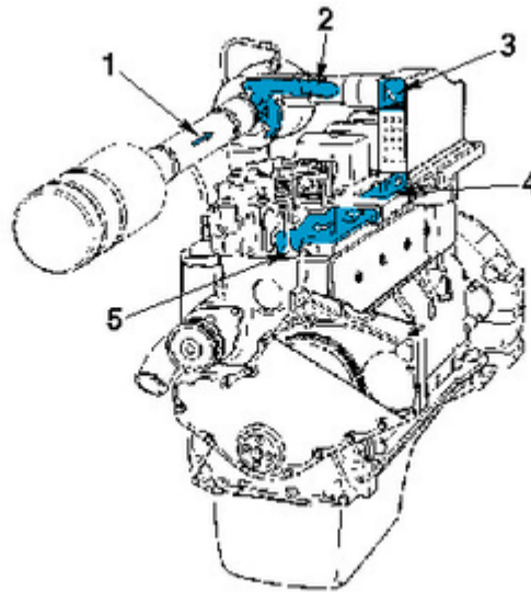
Turbocharged-Aftercooled Engine
