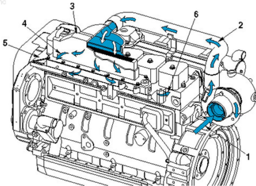
Jacket Water Aftercooled
