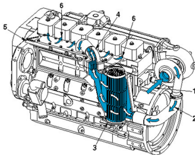
Sea Water Aftercooled
