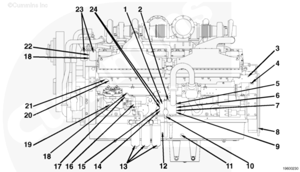
Left View - QSK45 similar and QSK60 (sensor locations)
