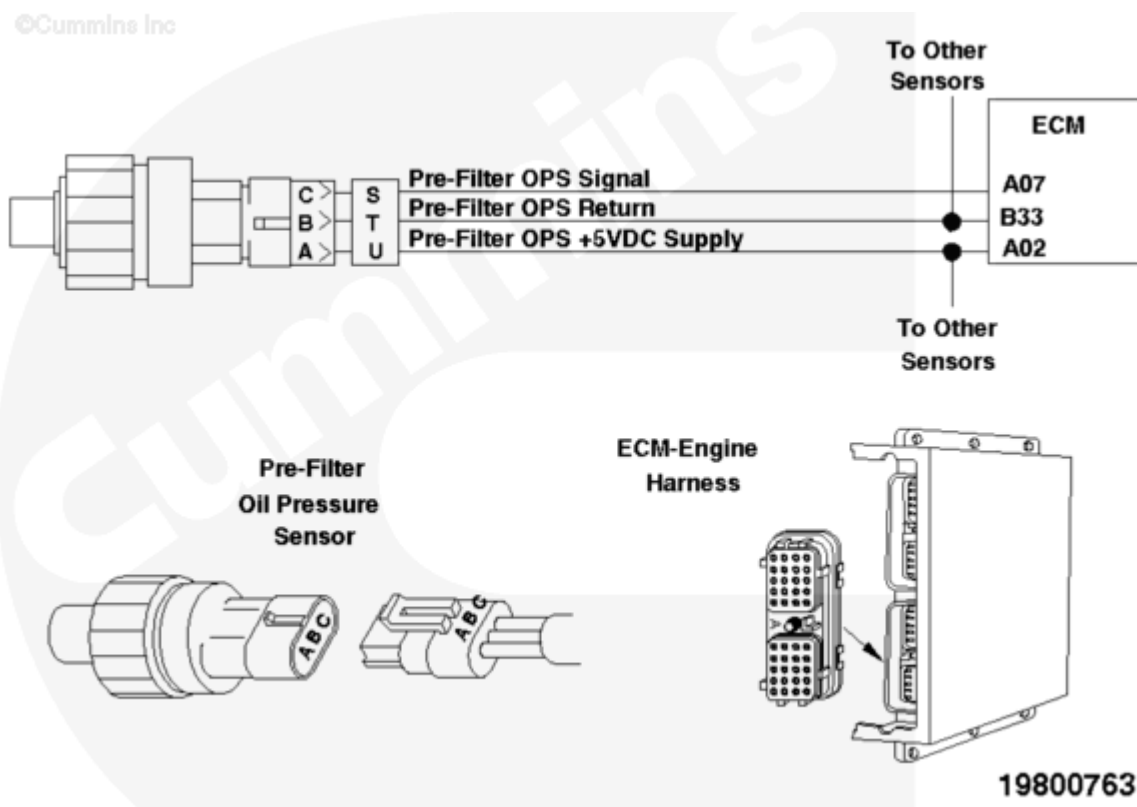
Prefilter Oil Pressure Sensor Circuit
