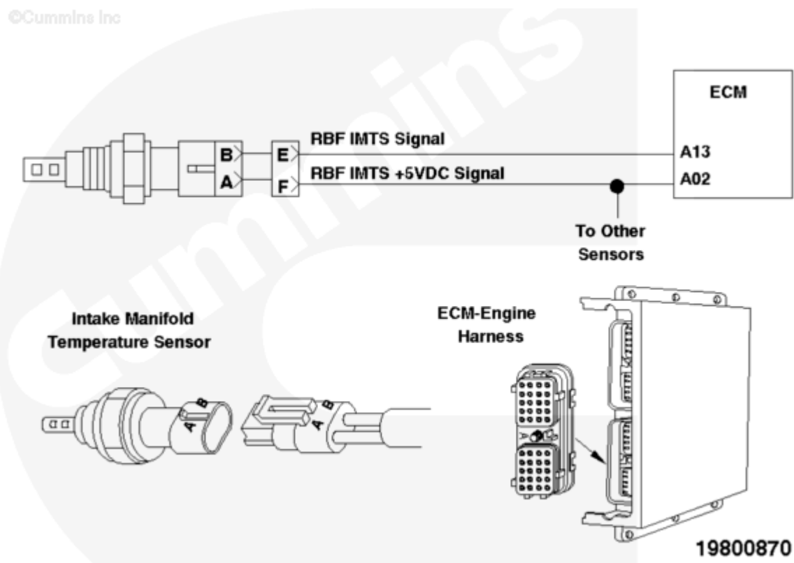
Right Bank Front Intake Manifold Temperature Sensor Circuit
