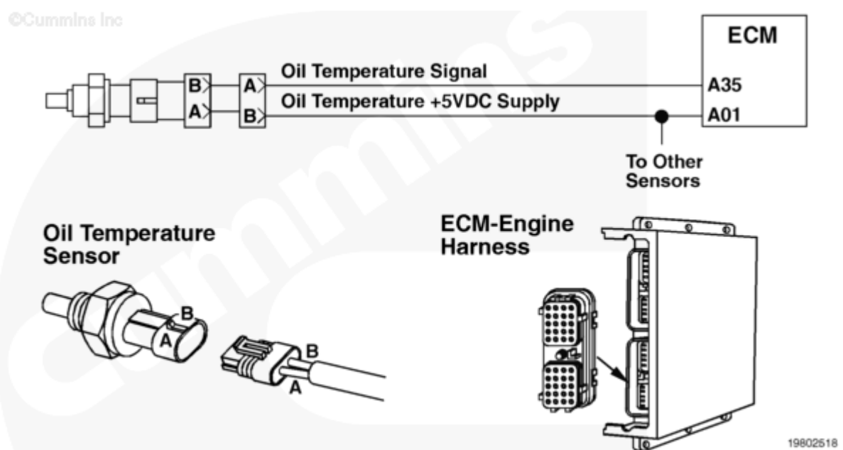
Oil Temperature Sensor Circuit
