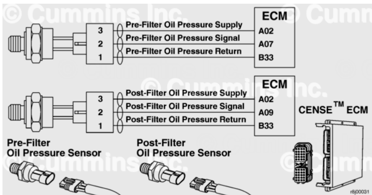
Pre-Oil Filter Pressure Sensor Circuit
