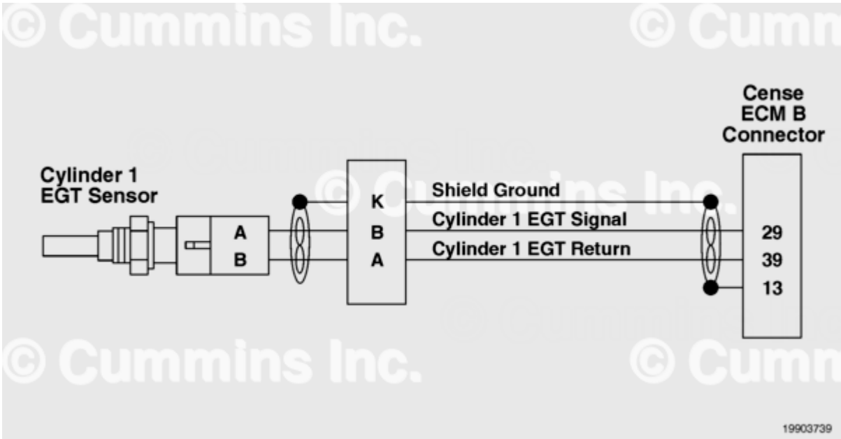
Exhaust Gas Temperature Sensor Circuit Cylinder 1
