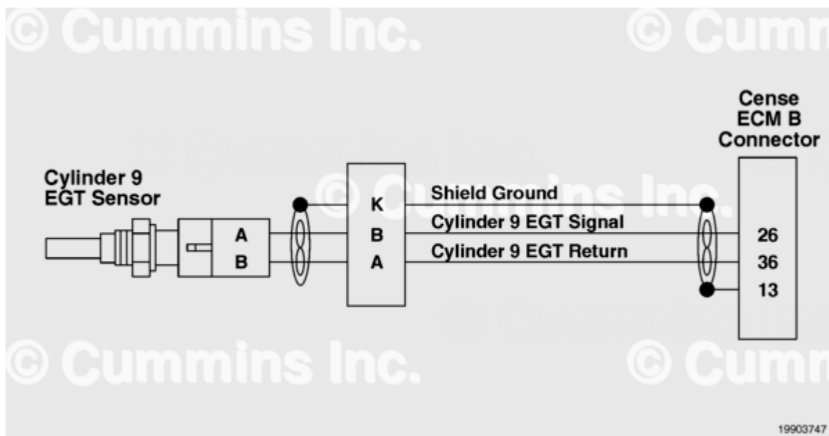
Exhaust Gas Temperature Sensor Circuit Cylinder 9
