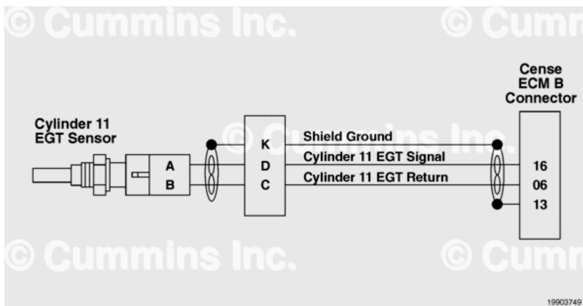
Exhaust Gas Temperature Sensor Circuit Cylinder 11
