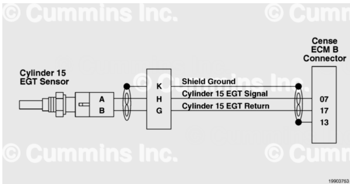
Exhaust Gas Temperature Sensor Circuit Cylinder 15
