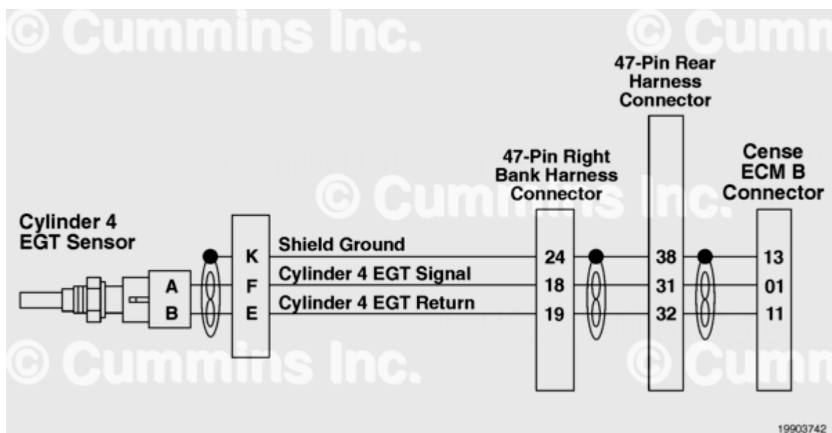
Exhaust Gas Temperature Sensor Circuit Cylinder 4
