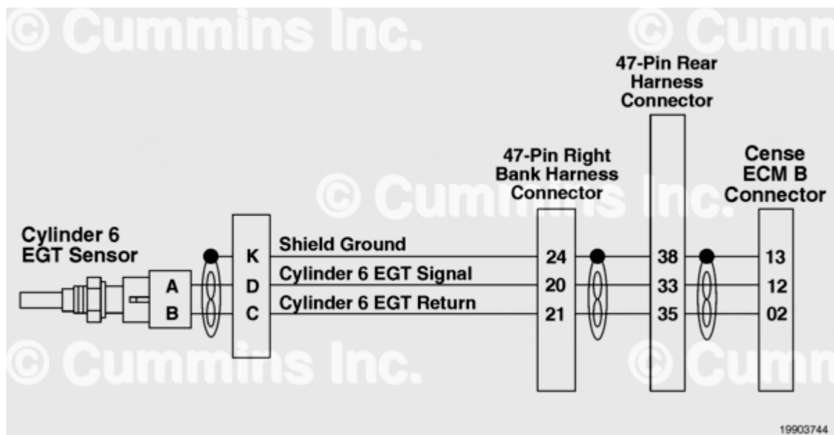
Exhaust Gas Temperature Sensor Circuit Cylinder 6
