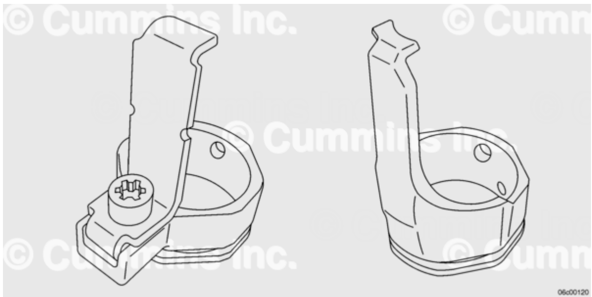
Old injector load ring (left) and new injector load ring (right)
