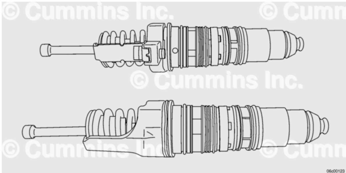
Old load ring on injector (top) and new load ring on injector (bottom)
