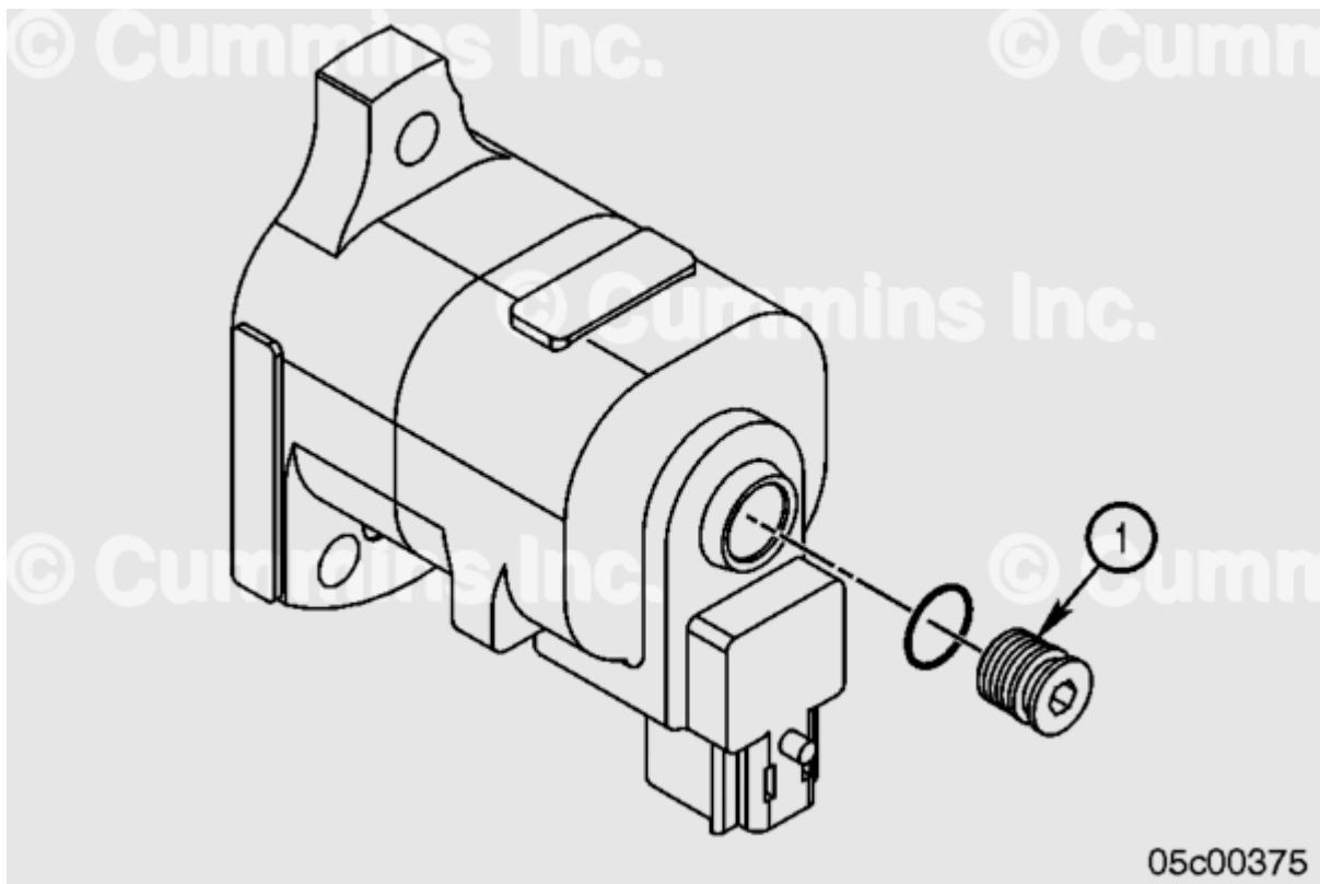
Plug with o-ring seal (1) - Design 2
