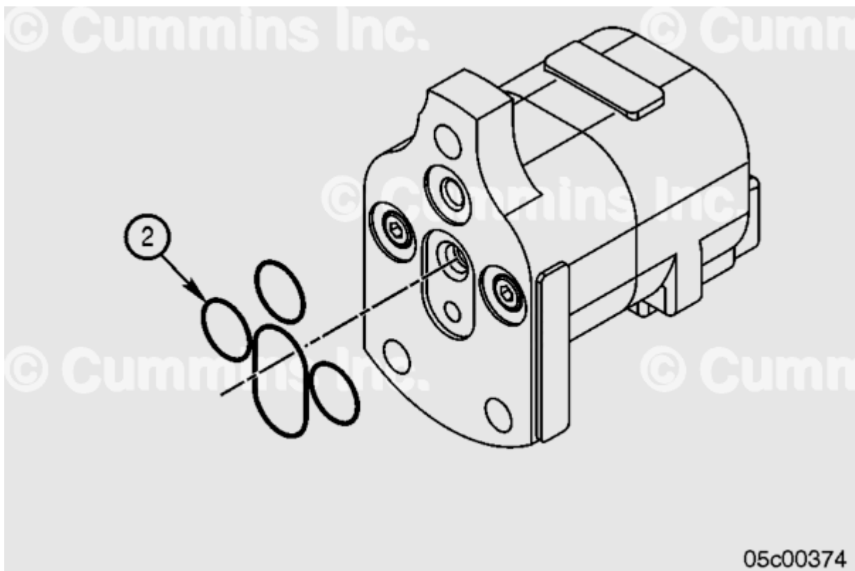
O-ring type mounting gasket (2) - Design 1
