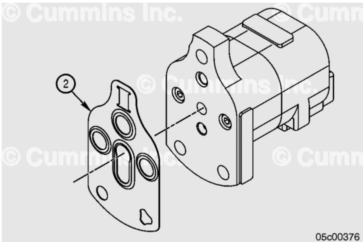
Embossed steel mounting gasket (2) - Design 2
