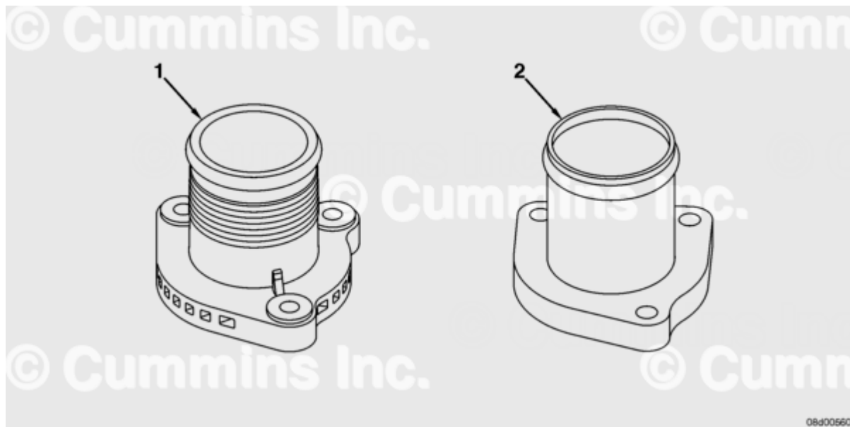
Figure1 - New Part Number 5261014 and Figure 2 - Old Part Number 3943300
