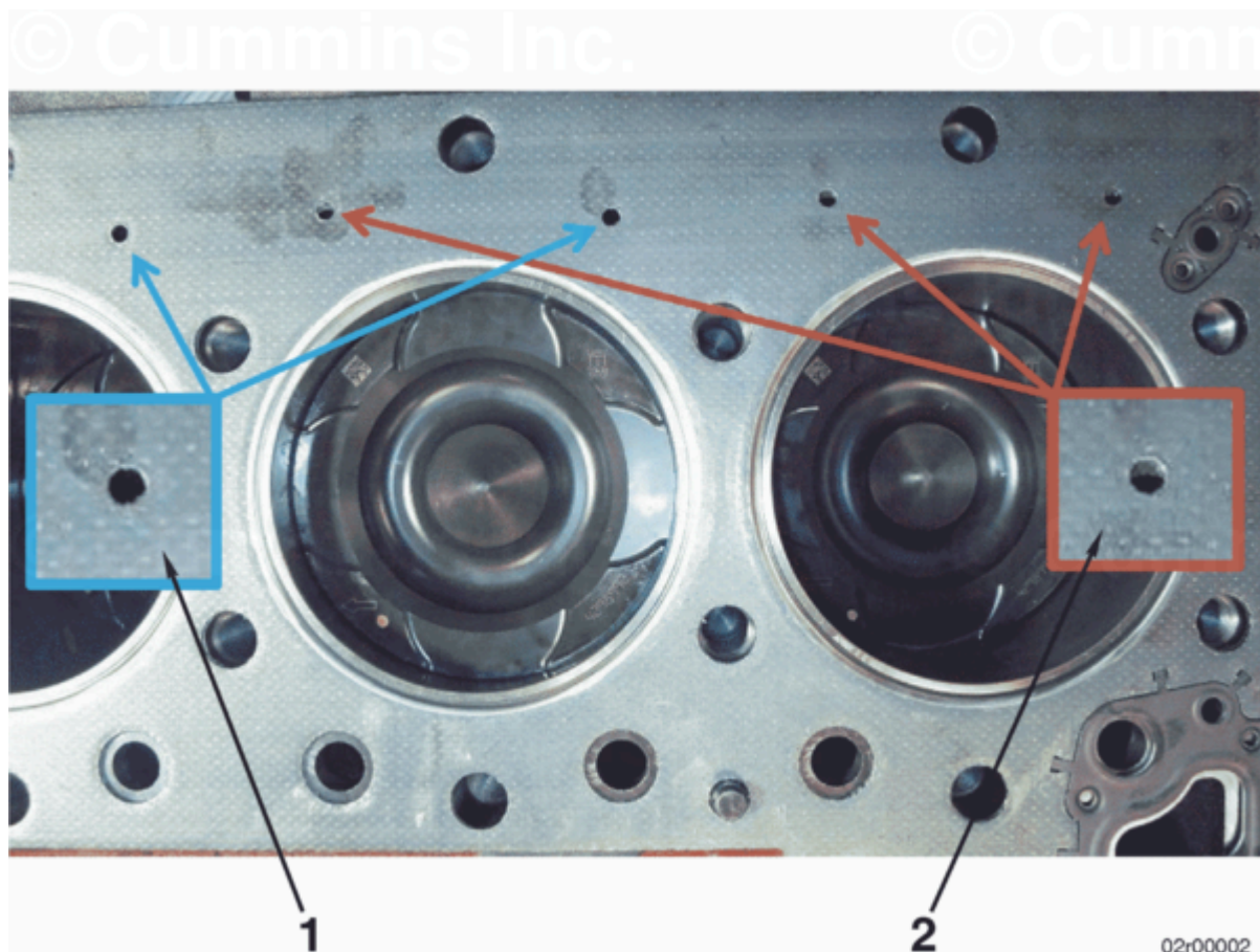
Figure 1, New Cylinder Head Gasket on Cylinder Block
