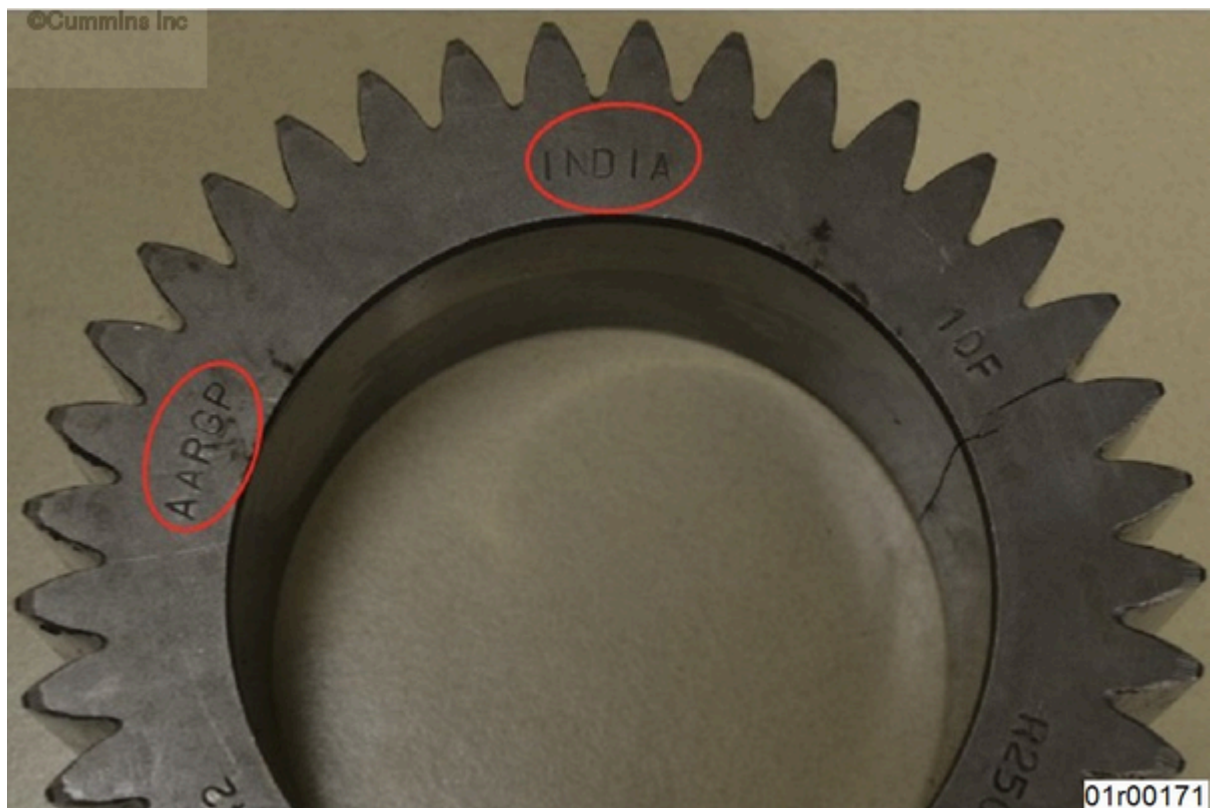
Figure 1, Identification Marks on the Rear Face of Suspect Crankshaft Gear
