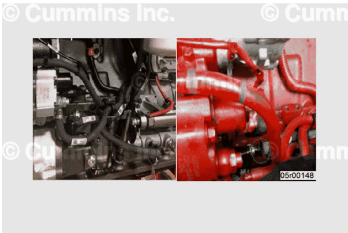
Figure 3, Location of Fuel Supply Tube Malfunction.
