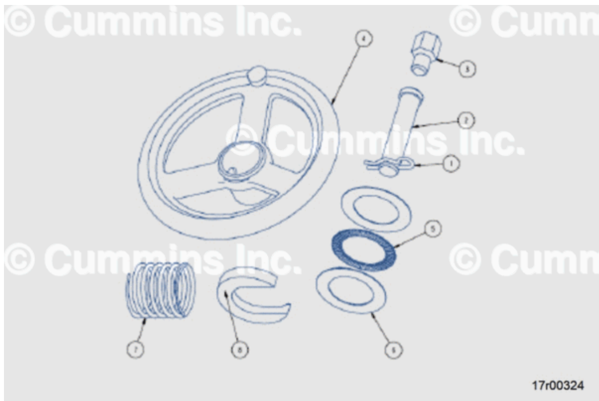
Figure 1, Counterbore Cutting Improvement Kit, Part Number 5395552.
