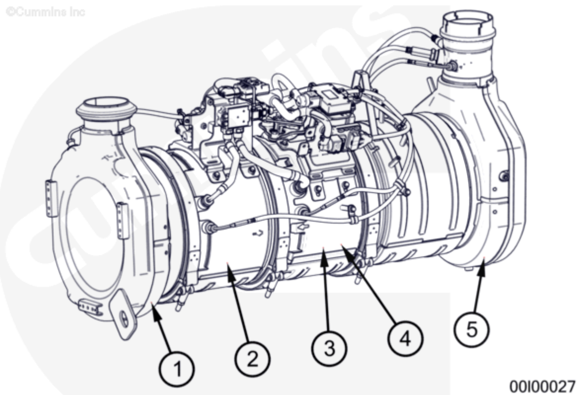
Figure 2, Aftertreatment Identification Location.
