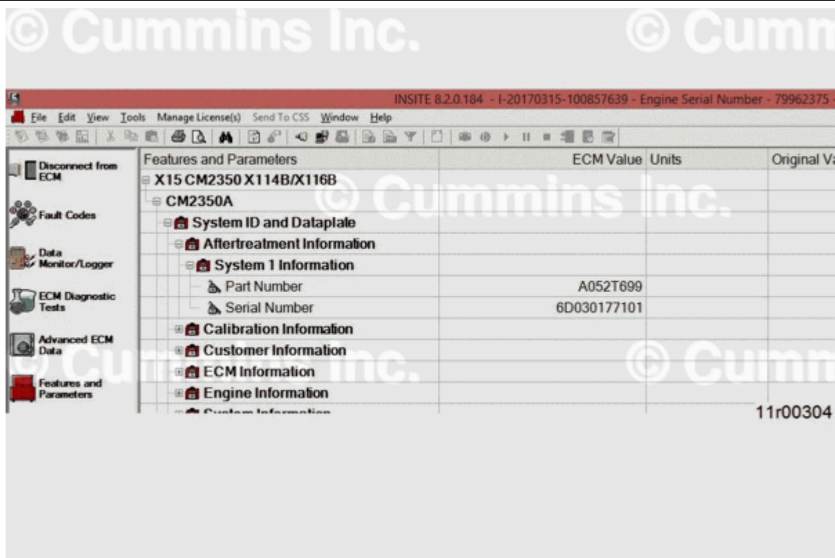
Figure 1, Aftertreatment Assembly Identification Numbers.
