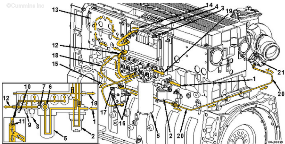
ISX With Lift Pump and Aftertreatment
