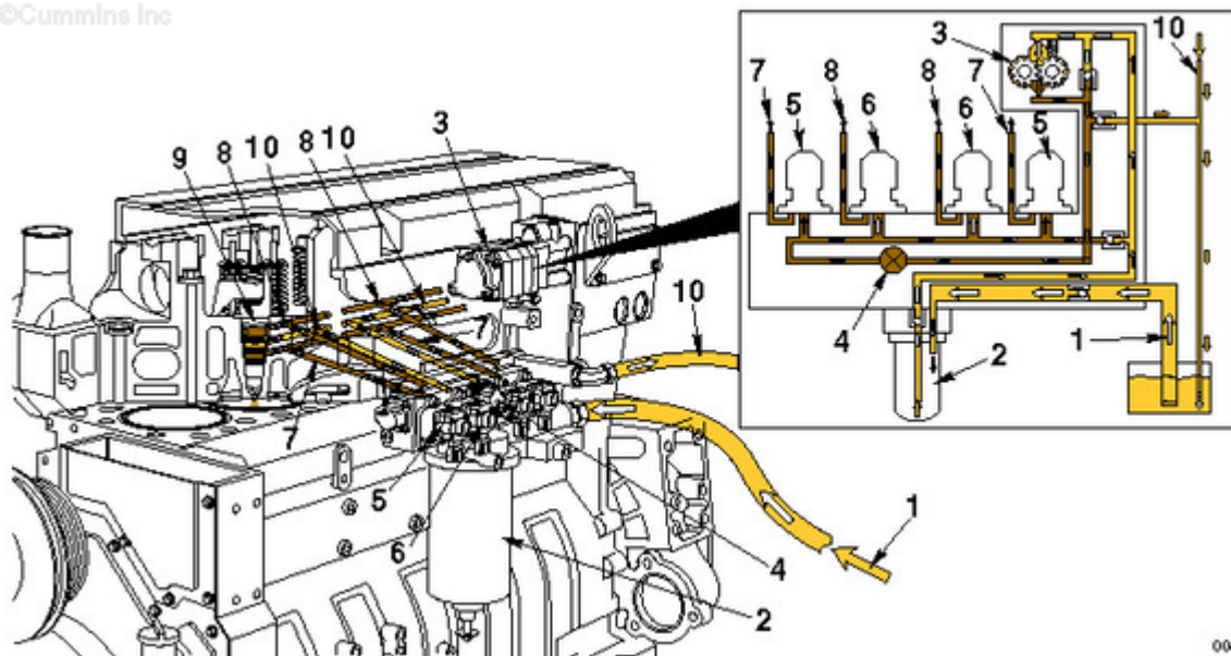
Without Lift Pump
