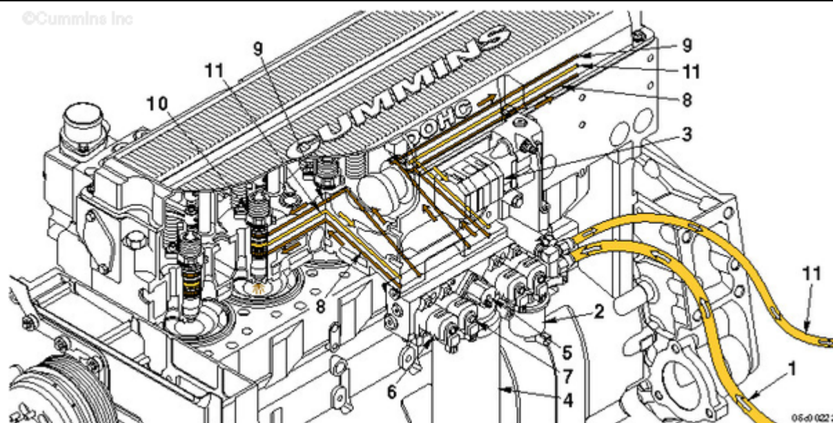
QSX15 With Lift Pump
