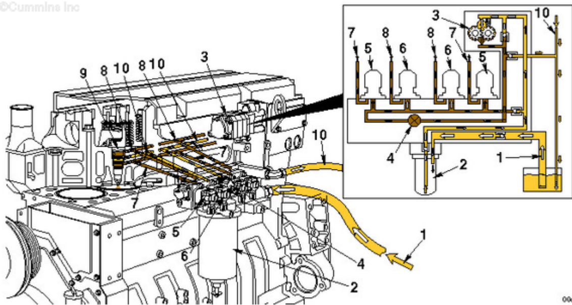
QSX15 Without Lift Pump
