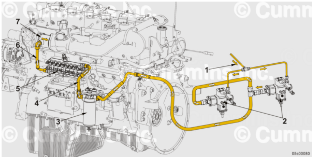
Compressed Natural Gas (CNG) Engine
