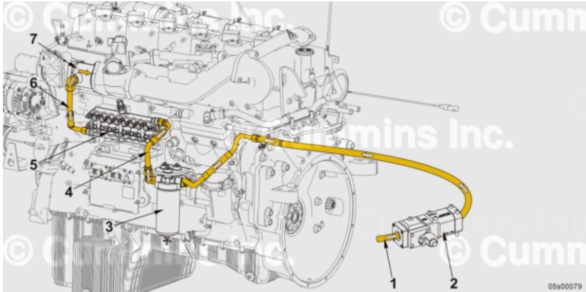
Liquefied Natural Gas (LNG) Engine
