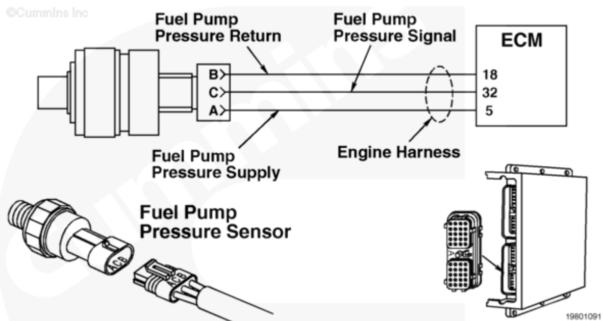
Fuel Pump Pressure Sensor Circuit
