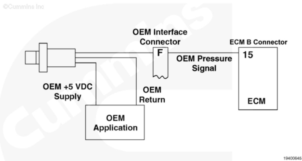
OEM Pressure Circuit
